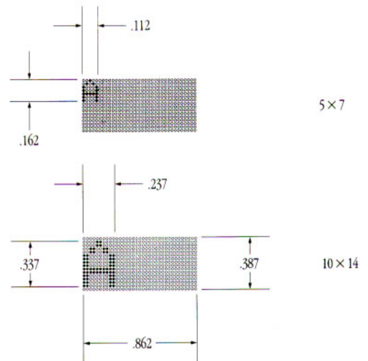
FIGURE 12 CHARACTER SIZES
